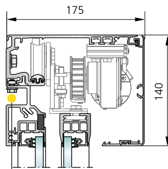
Header 140 mm (possible with supporting profile)
