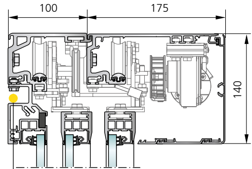
Header 140 mm telescopic (possible with supporting profile)
