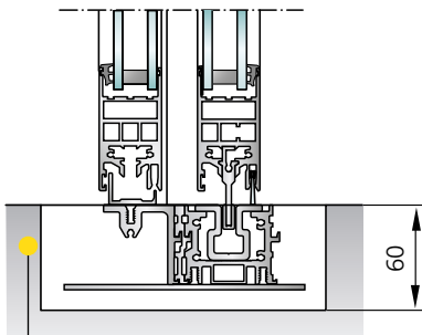
Full-length bottom rail integrated in the floor (for increased safety and stability), bottom rail with drainage optionally available
