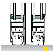
Lateral fixed point guide on the floor
