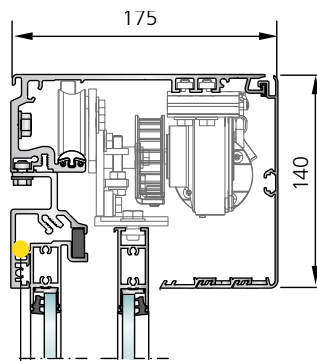
Header 140 mm with side panel (possible with supporting profile)
